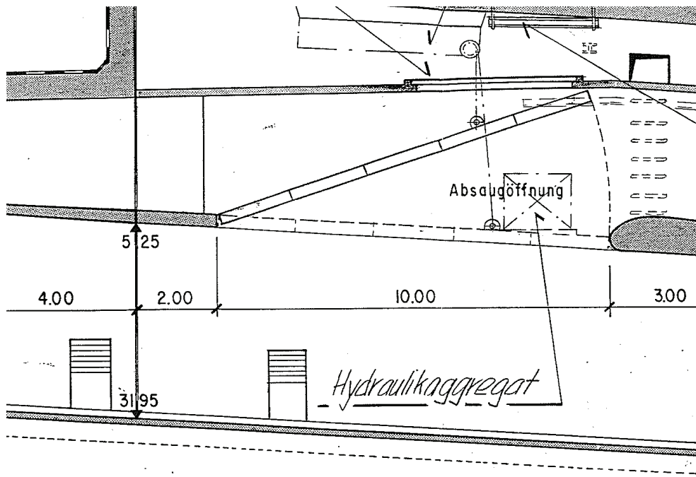
Figure 3.3: Longitudinal section of flap gate
