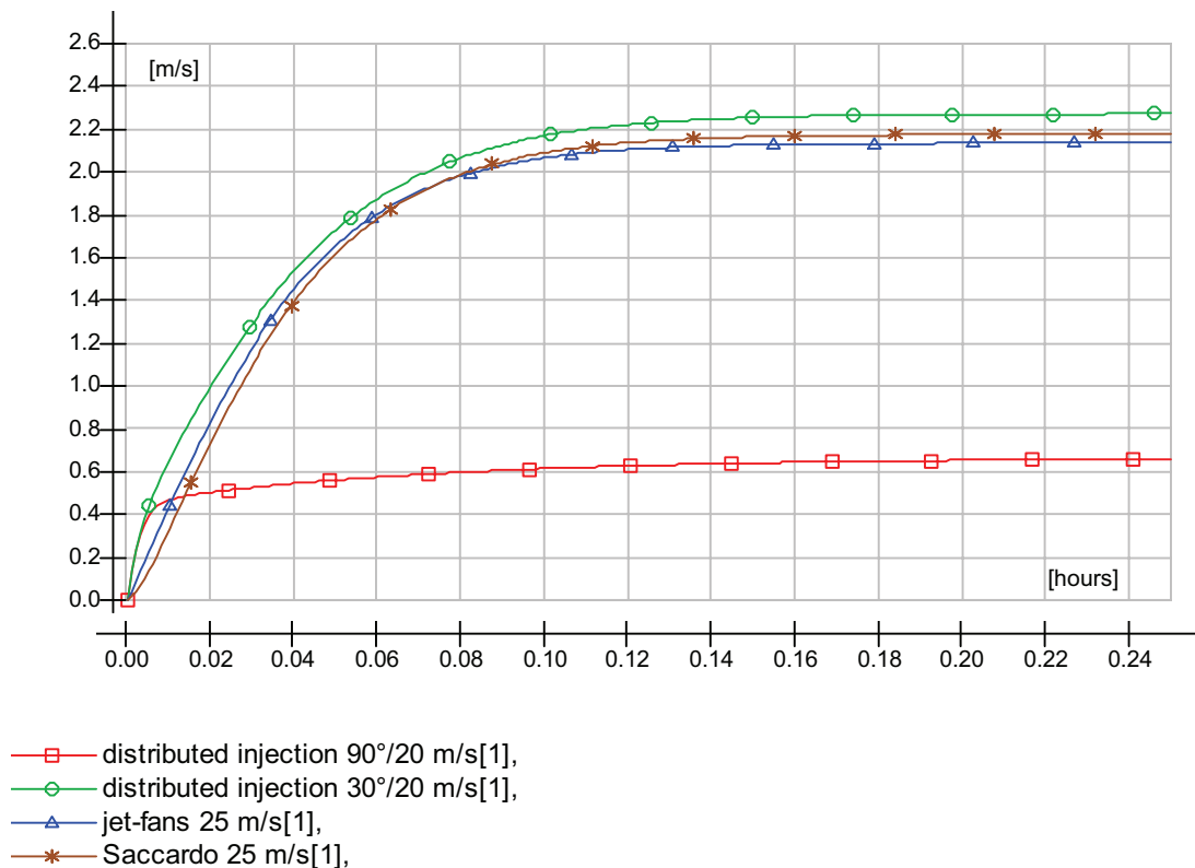
Figure 3.8: Calculated air velocities in tunnel for the four different propulsion methods.
