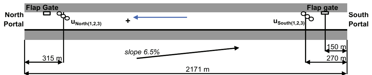
Figure 3.4: Location of anemometers and flap gates.
