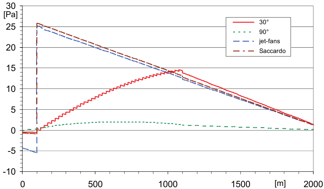
Figure 3.9: Distribution of static pressure along tunnel axis
