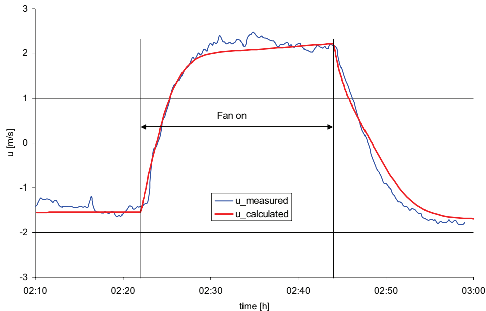
Figure 3.7: Air velocity in tunnel during operation of Saccardo nozzle.
