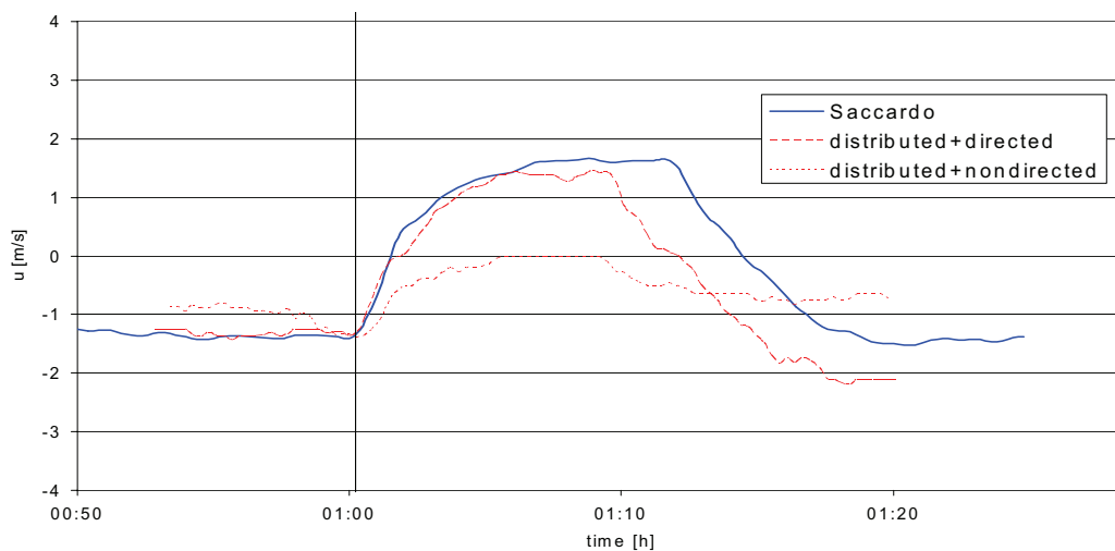
Figure 3.10: Qualitative comparison of propulsion methods in full scale experiment
