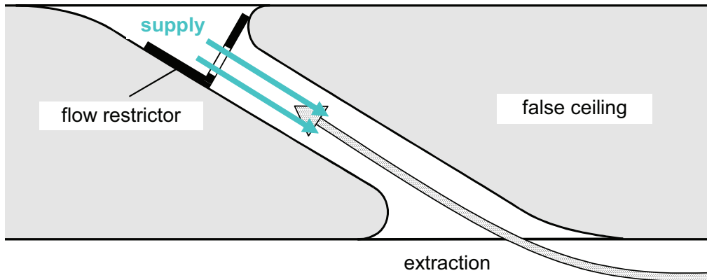
Figure 3.1: Sketch of openings for distributed injection/extraction in false ceiling
